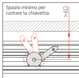
Portarullo standard
