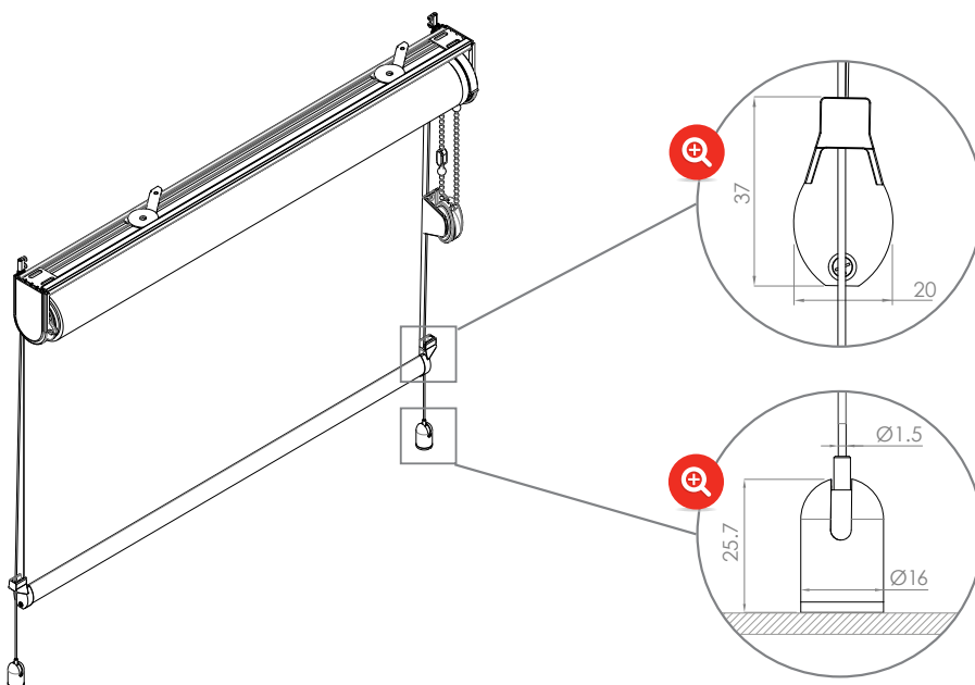
Portarullo standard
